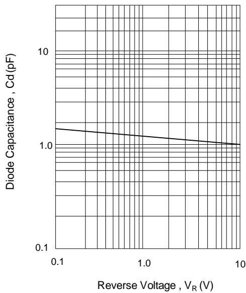
Diode capacitance VS. Reverse Voltage
